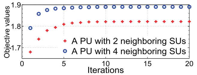
(a) Fast convergence of Distributed Bargaining for FLEC.
