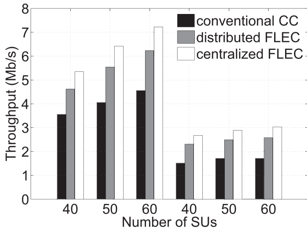
Fig. 3. Overall throughput performances. The first three bars represent PU throughput, and the last three bars represent SU throughput.
