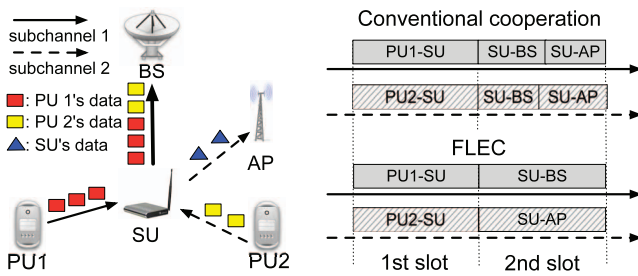
Fig. 1. The motivating scenario for Flexible Channel Cooperation .
